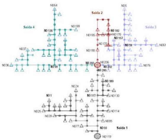
Fig. 2. Rural Medium Voltage Network
