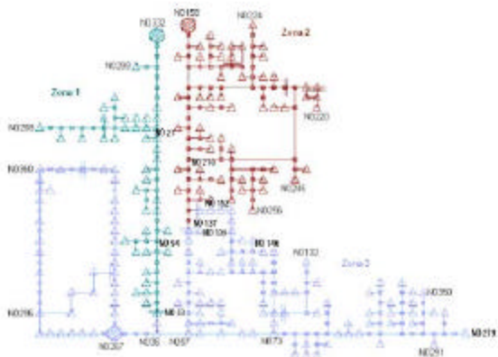
Fig. 3. Semi-Urban Medium Voltage Network
