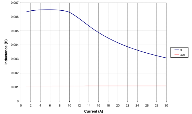
Fig. 8. Inductance versus current for the aligned and unaligned positions of the SRM
