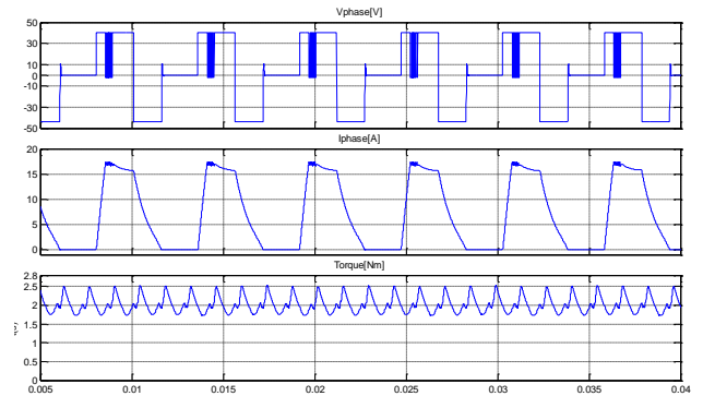
Fig. 13. Voltage, current and torque waveforms at 1800 rpm and current reference of 17 A
